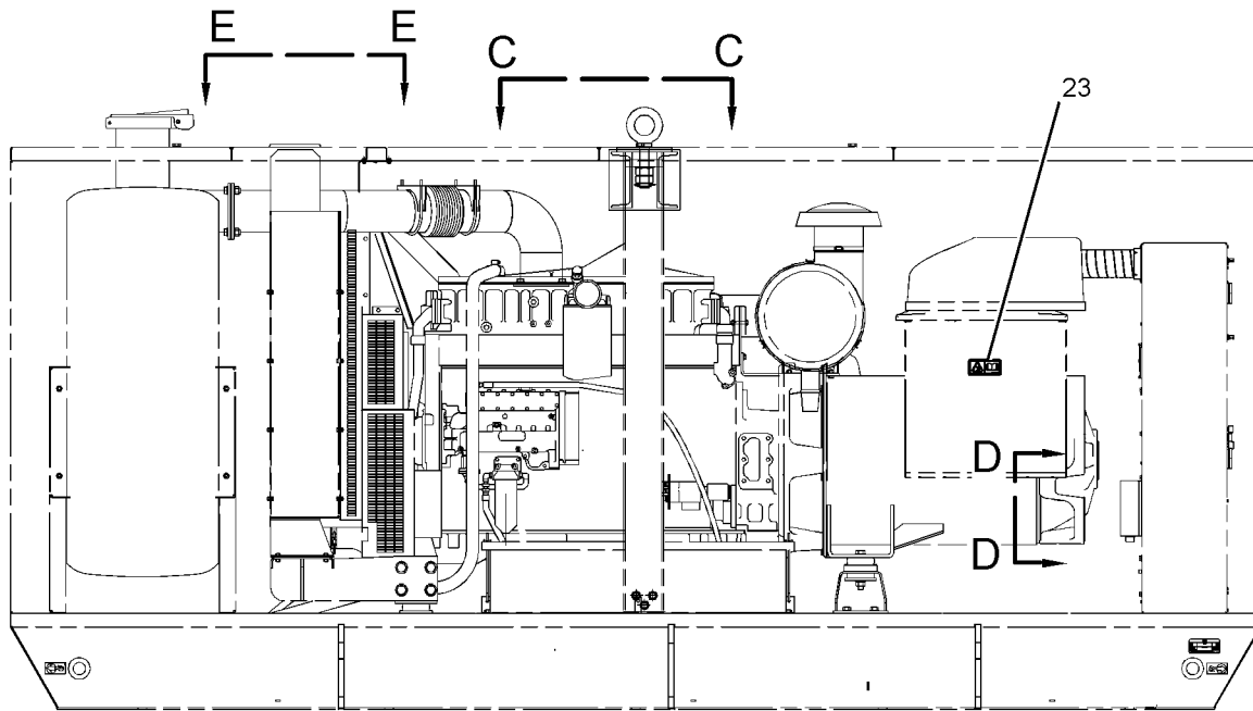
LEFT SIDE VIEW (ENGINE DETAIL)
