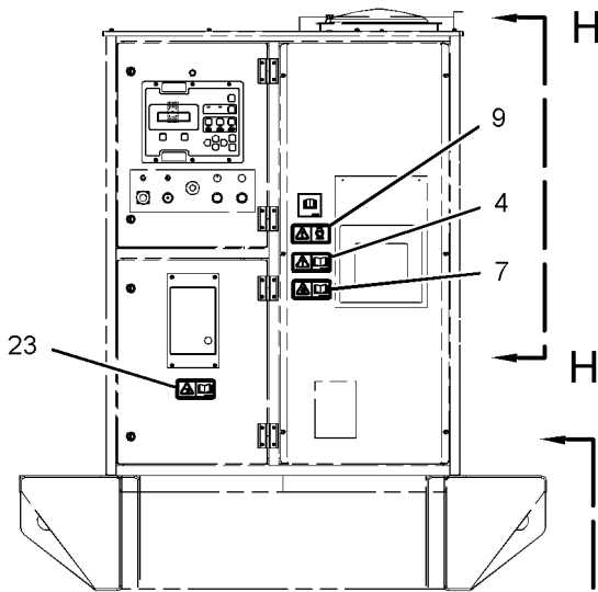
REAR VIEW (BREAKER DETAIL)
