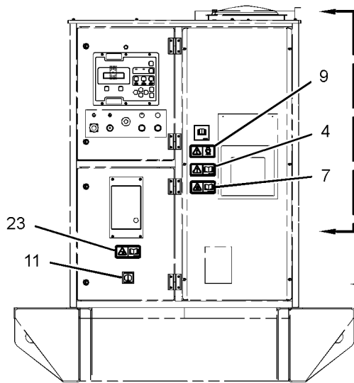
REAR VIEW (BREAKER DETAIL)
