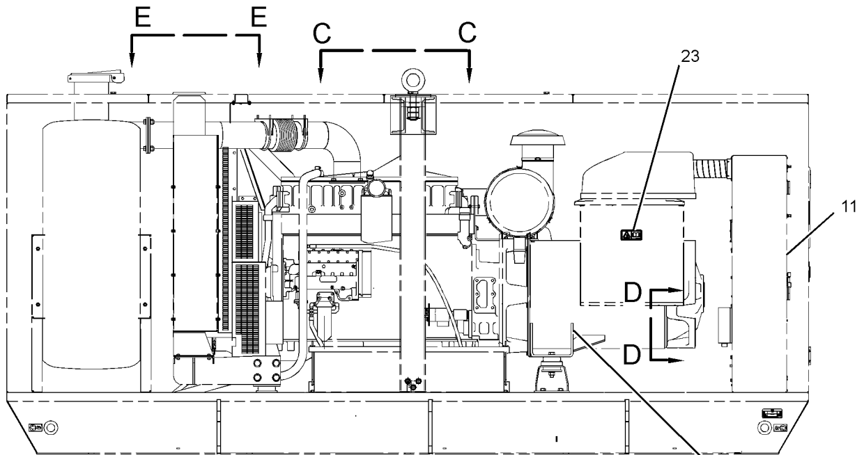
LEFT SIDE VIEW (ENGINE DETAIL)
